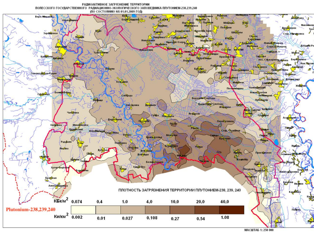
Figure A3: 2009 map of the surface ground deposition of plutonium-238,239,240 in the Belarussian part of the Chernobyl exclusion zone. The upper scale is in kBq/m 2 and the lower scale in Ci/km 2 .
