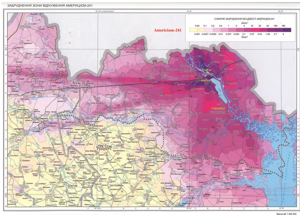
Figure A12: 2011 map of the surface ground deposition of americium-241 in the Ukrainian part of the Chernobyl exclusion zone. The upper scale is in kBq/m 2 and the lower scale in Ci/km 2 .
