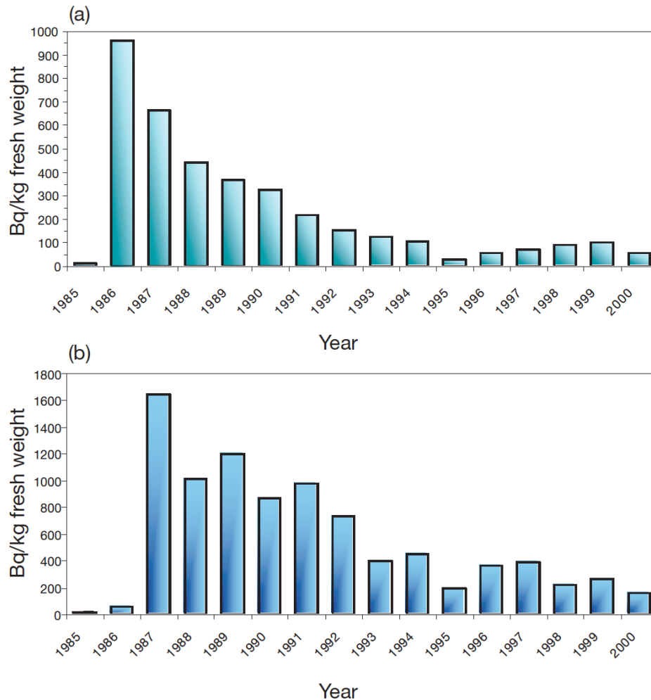
Figure 8: Averaged ^{137}\text{Cs} activity concentrations in nonpredatory (bream (a)) and predatory (pike (b)) fish; the fish are from the Kyiv reservoir. Figure reproduced from [IAEA2006b].
