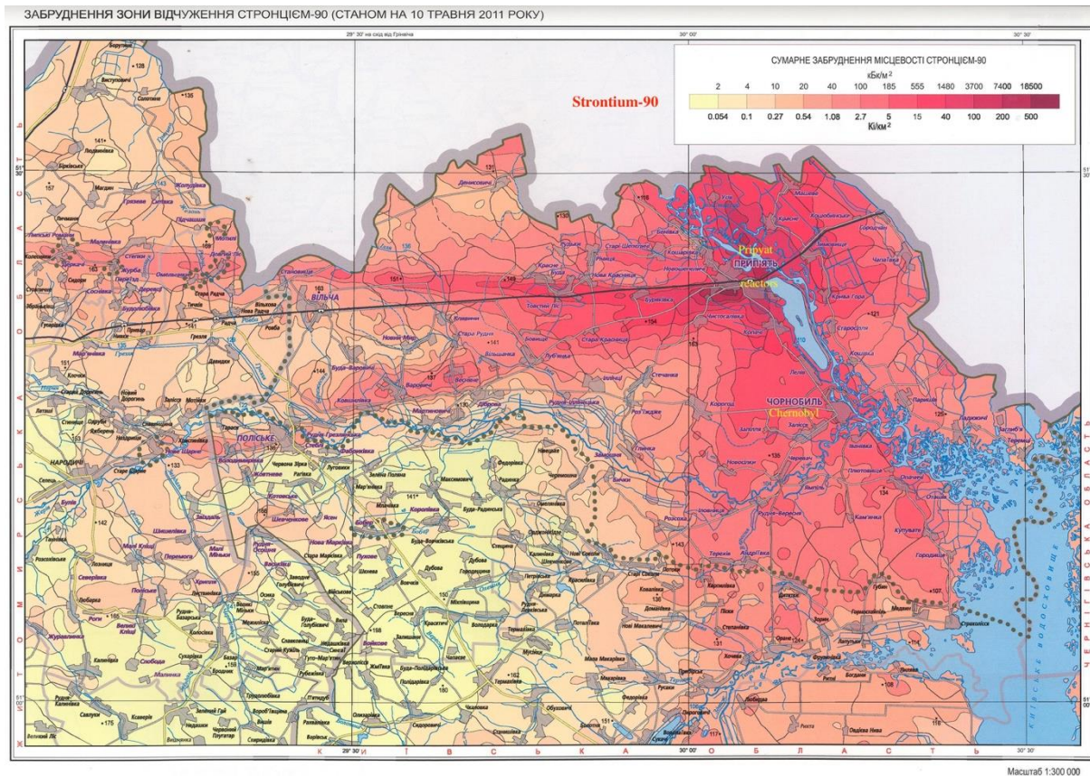
Figure A10: 2011 map of the surface ground deposition of strontium-90 in the Ukrainian part of the Chernobyl exclusion zone. The upper scale is in \text{kBq/m}^2 and the lower scale in \text{Ci/km}^2 .
