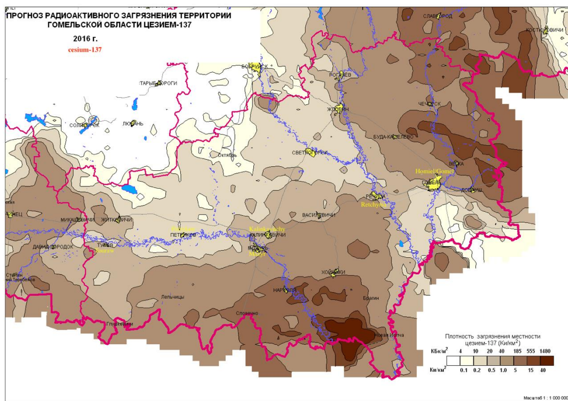
Figure A6: 2016 map of the surface ground deposition of cesium-137 in the Gomel oblast. The upper scale is in \text{KBq/m}^2 and the lower scale in \text{Ci/km}^2 .
