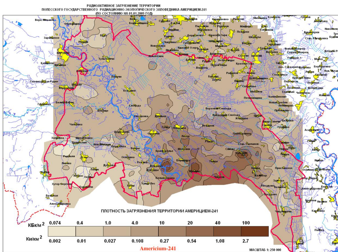
Figure A5: 2009 map of the surface ground deposition of americium-241 in the Belarusian part of the Chernobyl exclusion zone. The upper scale is in kBq/m² and the lower scale in Ci/km².
