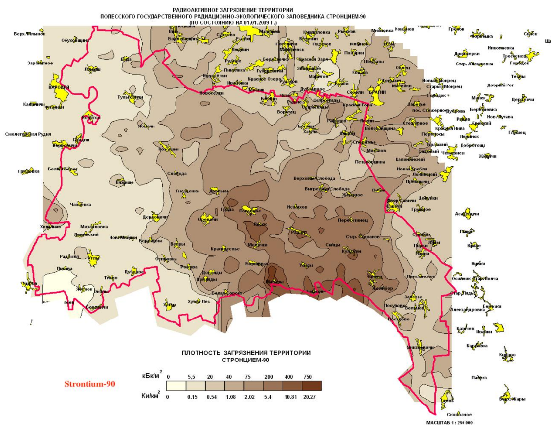
Figure A2: 2009 map of the surface ground deposition of strontium-90 in the Belarusian part of the Chernobyl exclusion zone. The upper scale is in kBq/m² and the lower scale in Ci/km².
